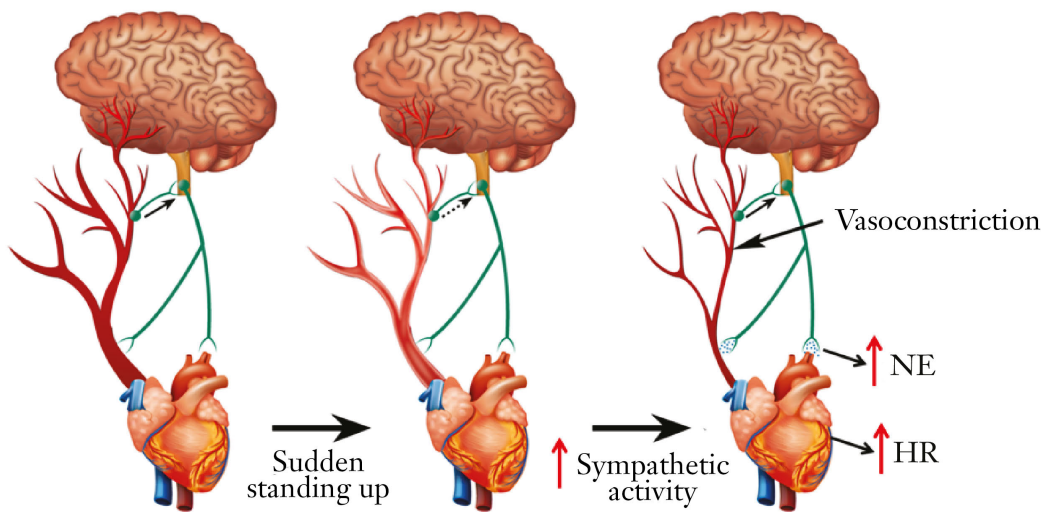
FIGURE 2.19. Baroreflex pathway.
